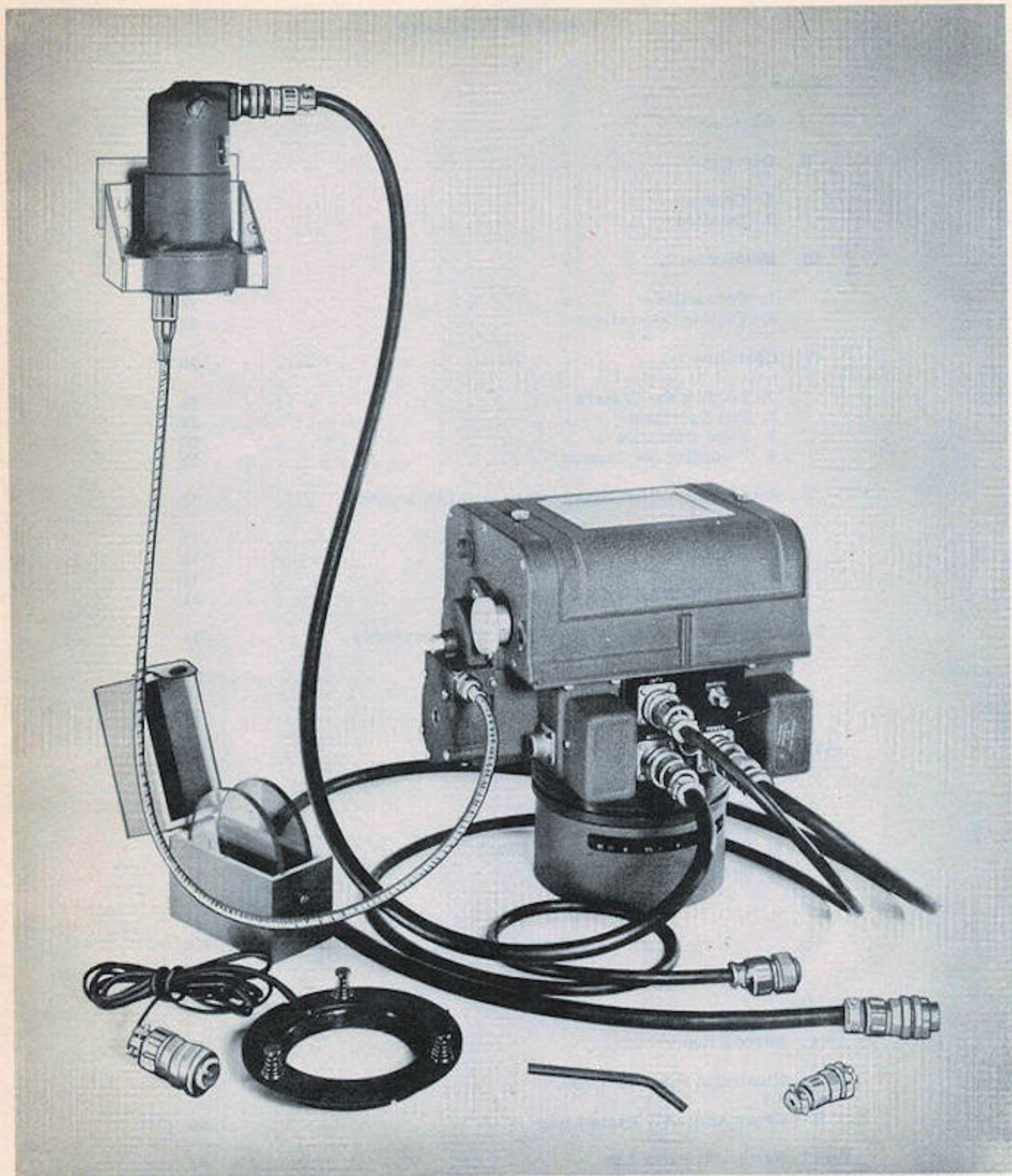
Figure 1 - Type K-21 Aircraft Camera and Equipment
